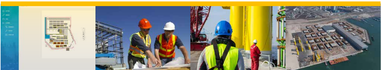
IT Services
